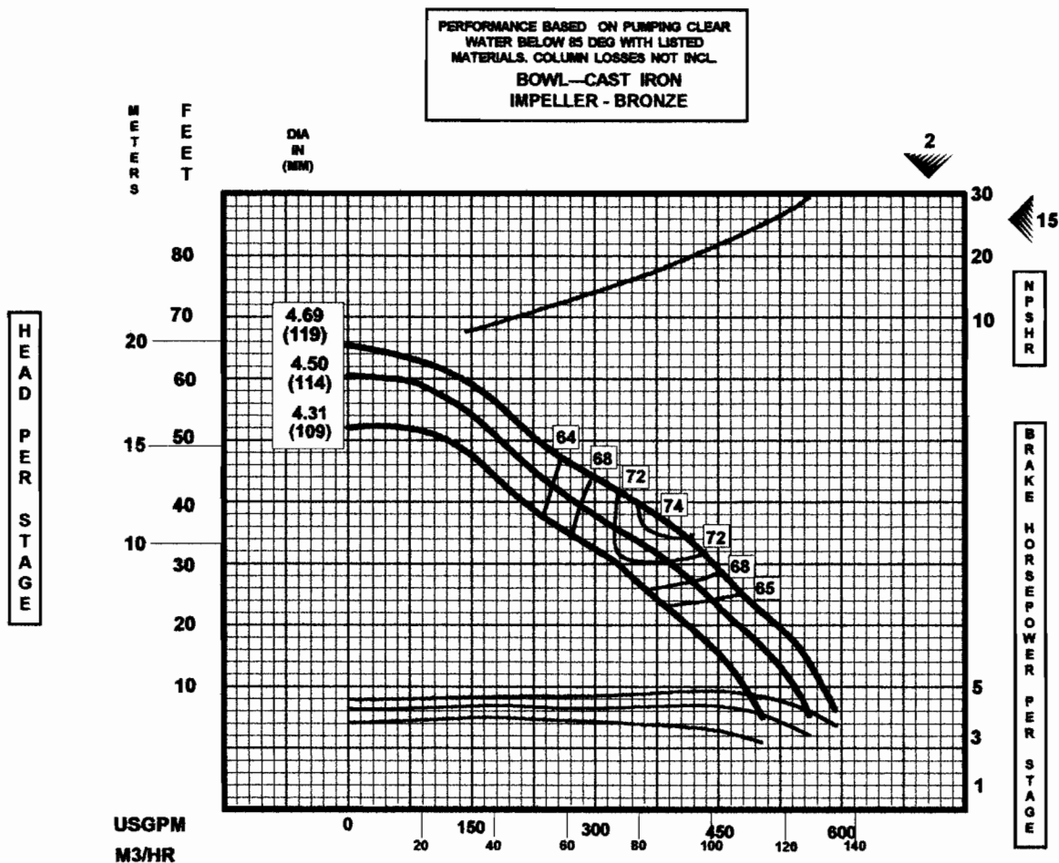
THRUST FACTORS AT BEP
