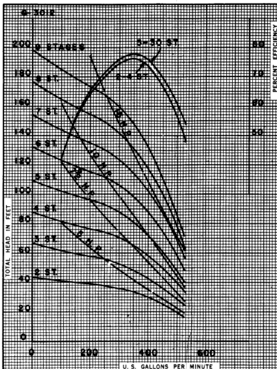
10" FIG. 6920 1160 RPM. MAXIMUM STAGES 30 IMPELLER 737 BRONZE WKPUC
