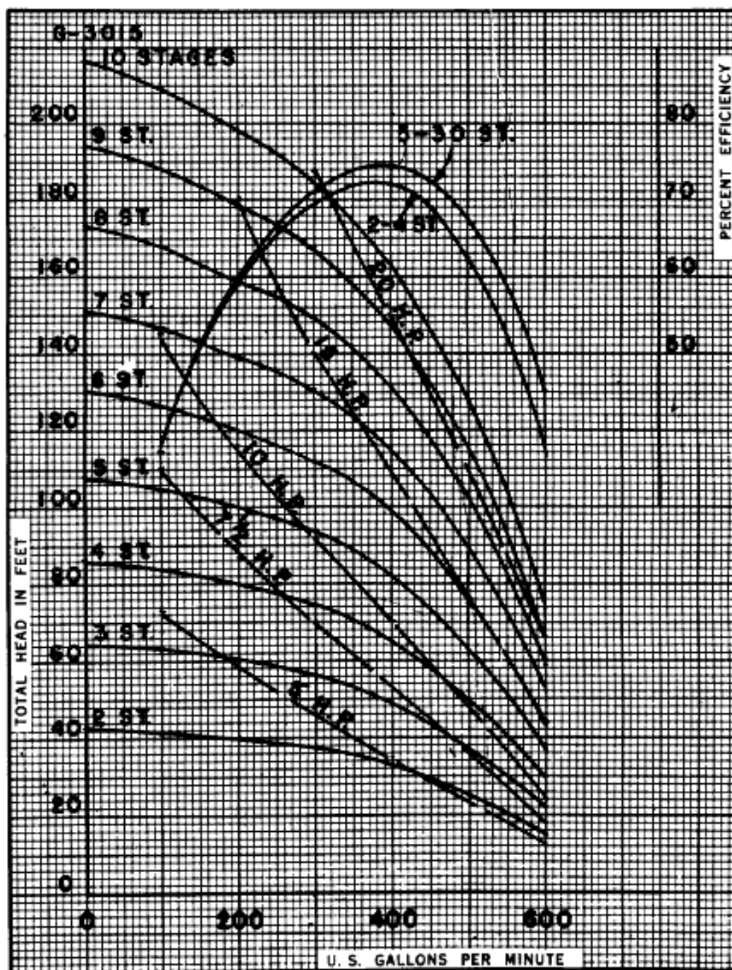
10" FIG. 6920 1160 RPM. MAXIMUM STAGES 30 IMPELLER 738 BRONZE WKPXF
