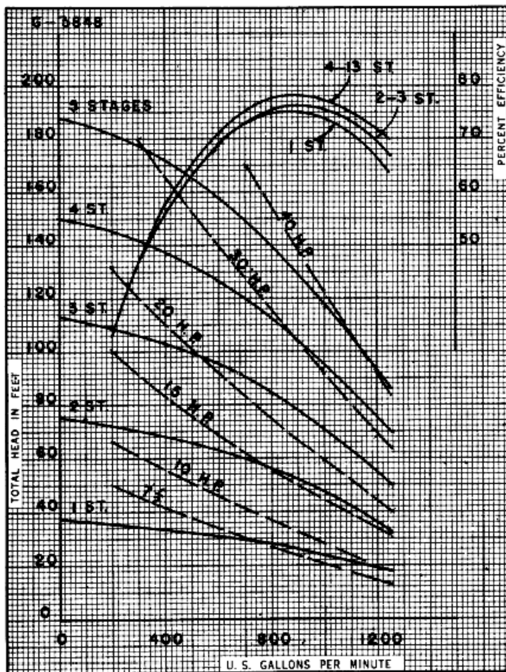
12" FIG. 6920 1160 RPM. MAXIMUM STAGES 13 IMPELLER 1134 BRONZE WPKCU
