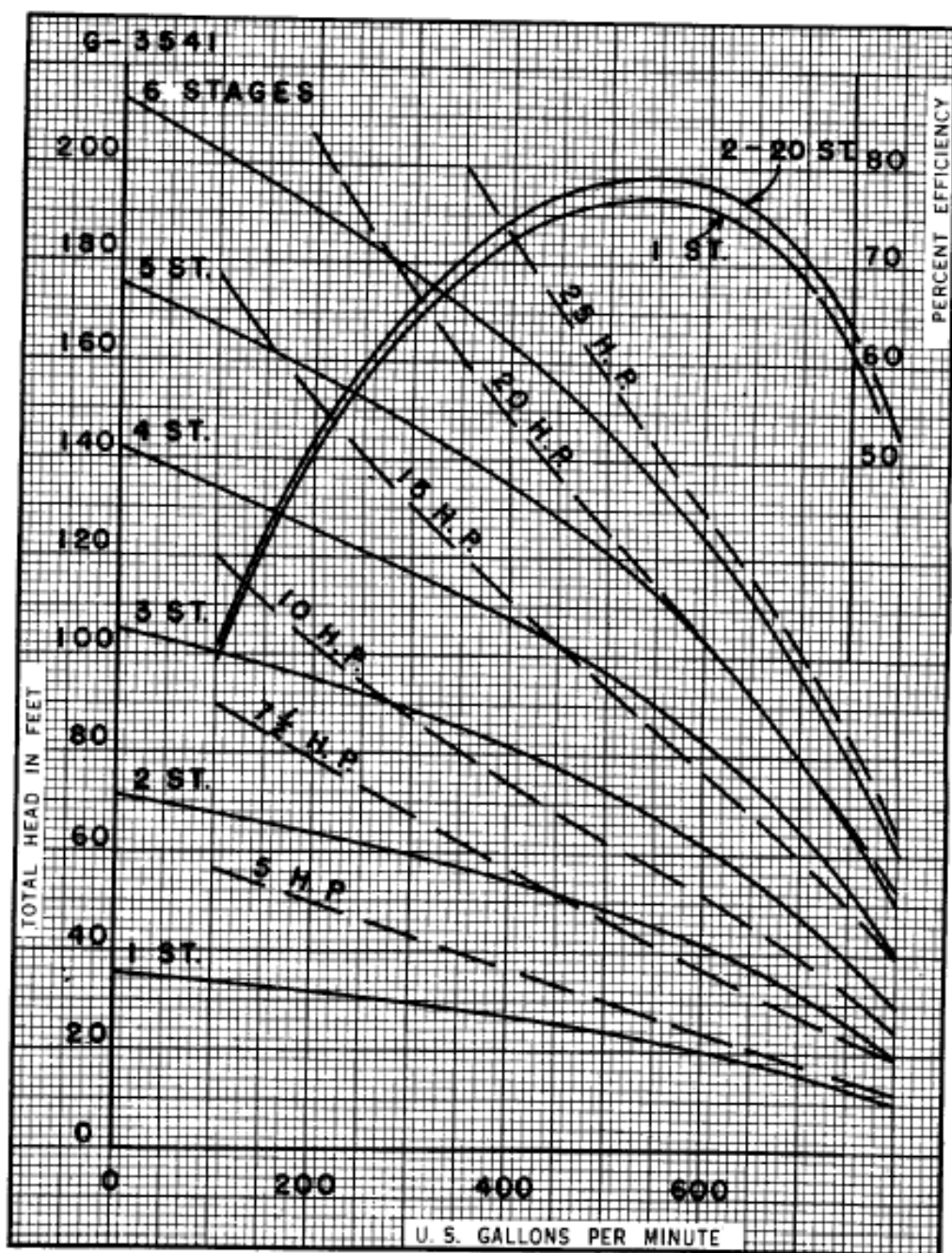
12" FIG. 6920 1160 RPM. MAXIMUM STAGES 20 IMPELLER 745 BRONZE WKVX
