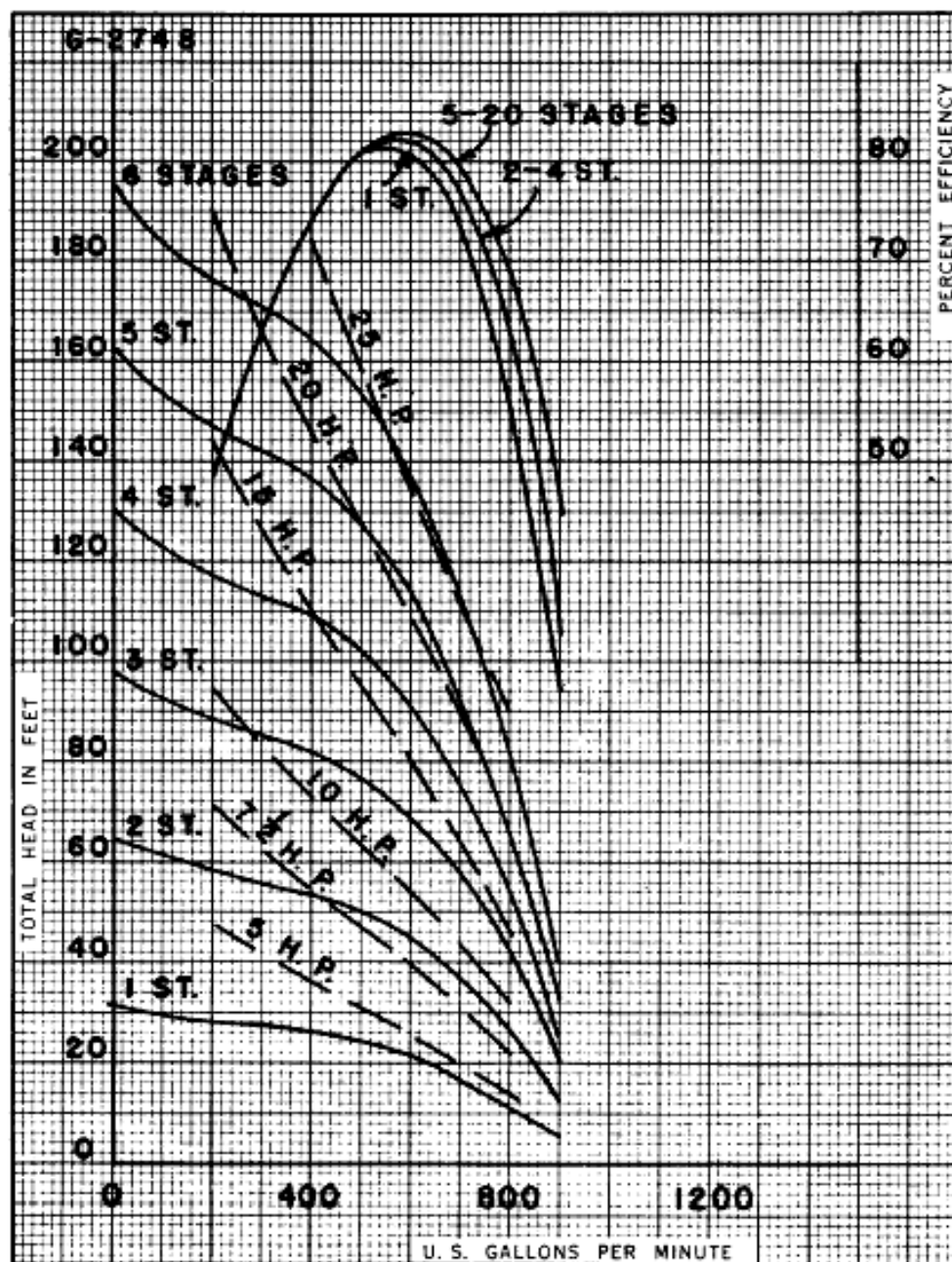
12" FIG. 6920 1160 RPM. MAXIMUM STAGES 20 IMPELLER 746 ALL ENAMELLED WKUMQ
