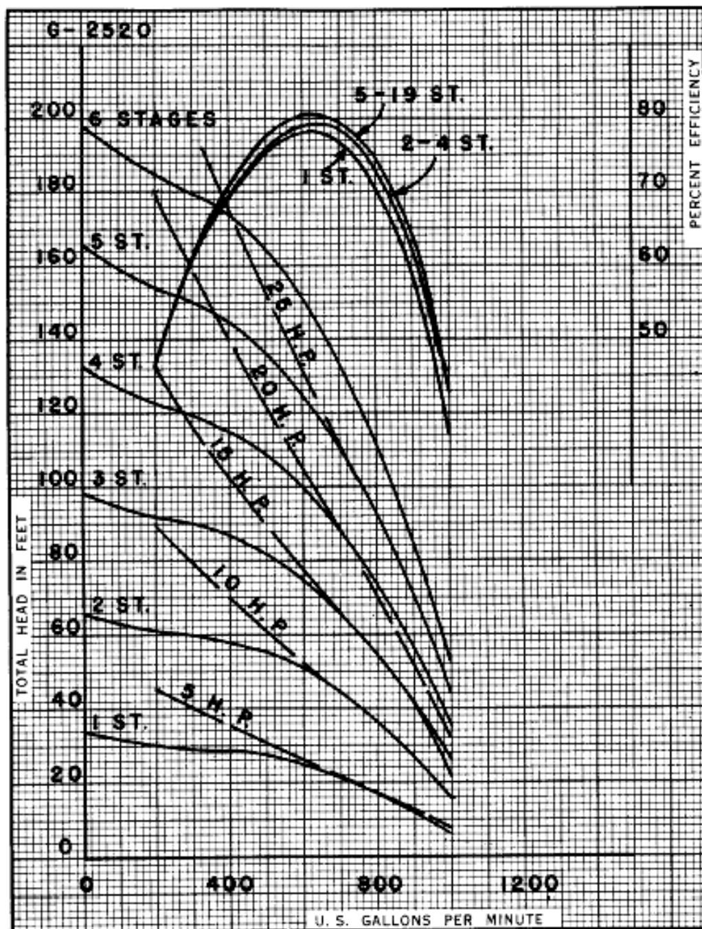
12" FIG. 6920 1160 RPM. MAXIMUM STAGES 19 IMPELLER 747 BRONZE WKUHL
