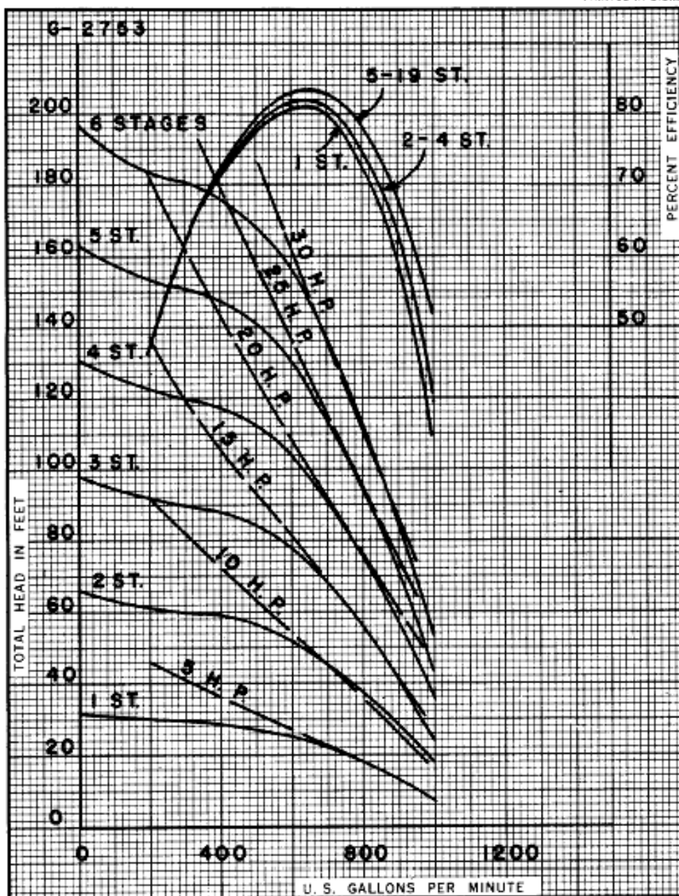
12" FIG. 6920 1160 RPM. MAXIMUM STAGES 19 IMPELLER 747 ALL ENAMELLED WKURY
