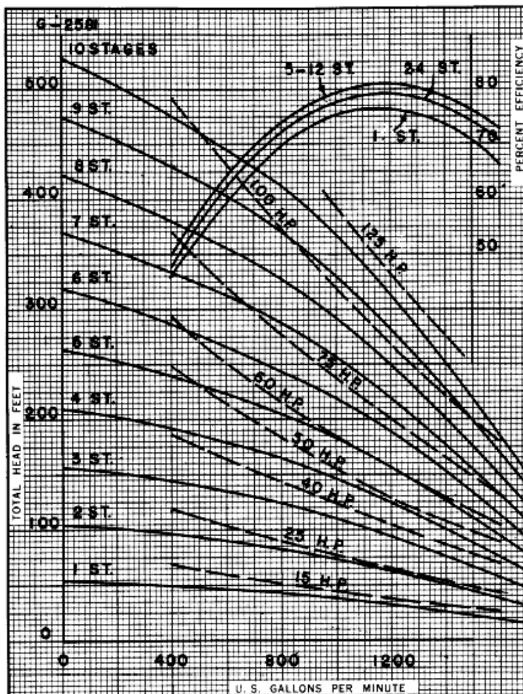
14" FIG. 6920 1160 RPM. MAXIMUM STAGES 12 IMPELLER 1203 BRONZE WKVBD
