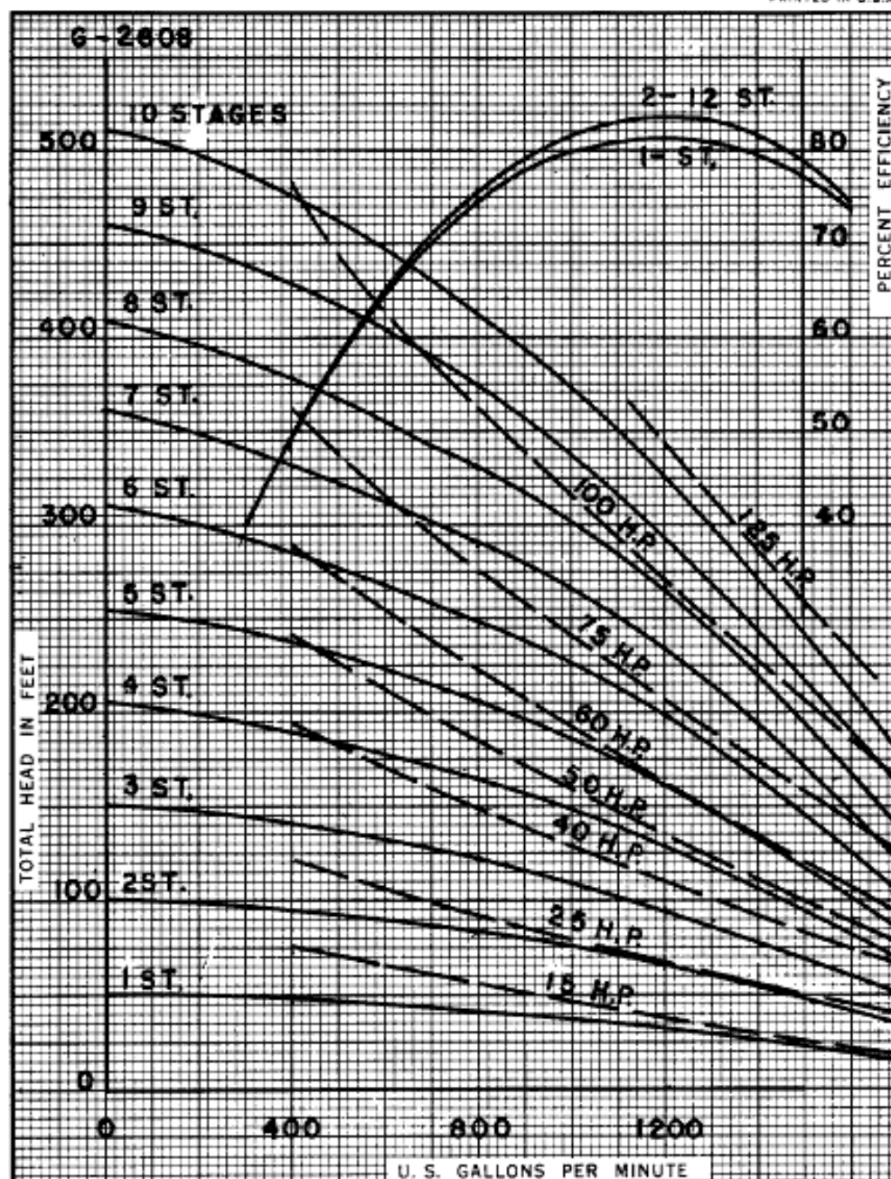
14" FIG. 6920 1160 RPM. MAXIMUM STAGES 12 IMPELLER 1203 ALL ENAMELLED WKVLO
