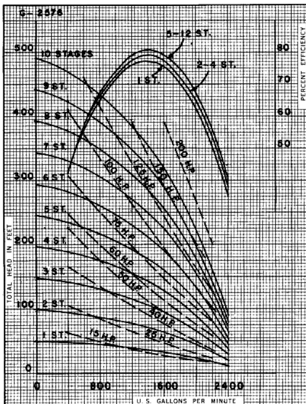
14" FIG. 6920 1160 RPM. MAXIMUM STAGES 12 IMPELLER 1204 BRONZE WKVGJ
