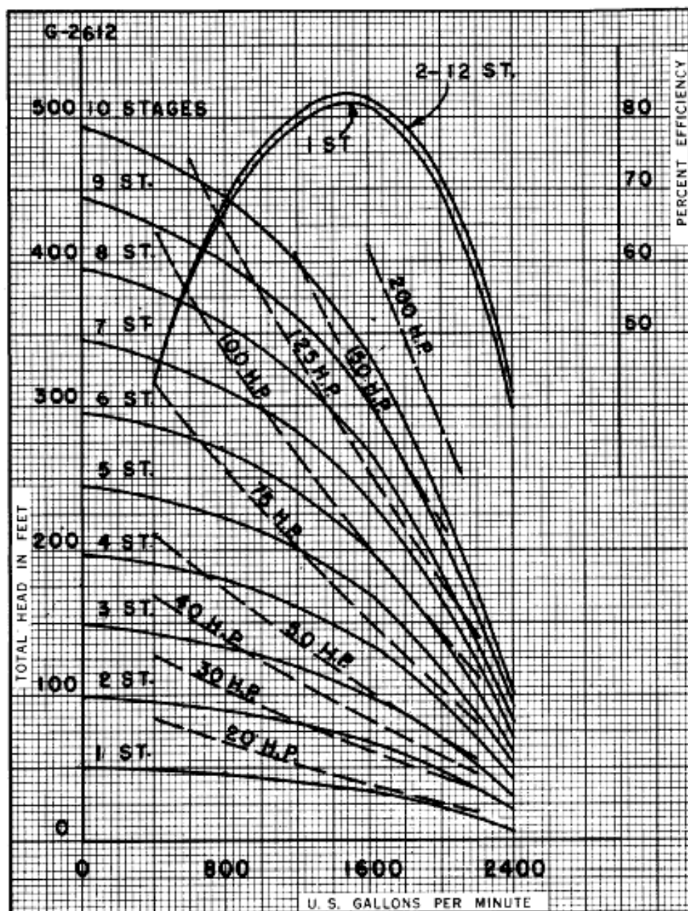
14" FIG. 6920 1160 RPM. MAXIMUM STAGES 12 IMPELLER 1204 ALL ENAMELLED WKVPS
