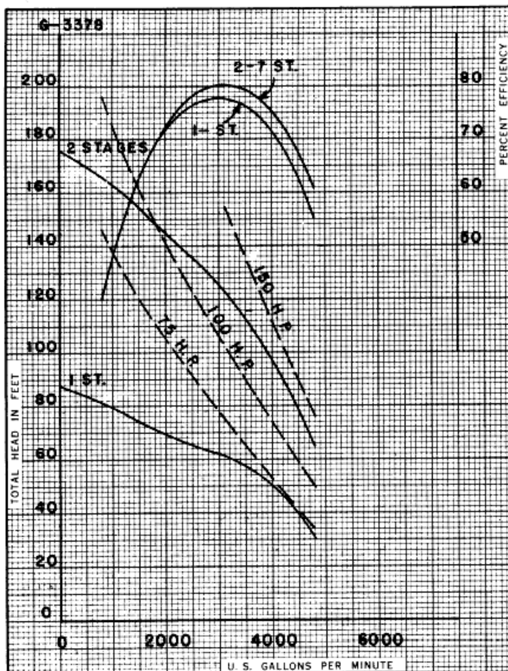
18" FIG. 6920 1160 RPM. MAXIMUM STAGES 7 IMPELLER 1214 BRONZE WKVSV
