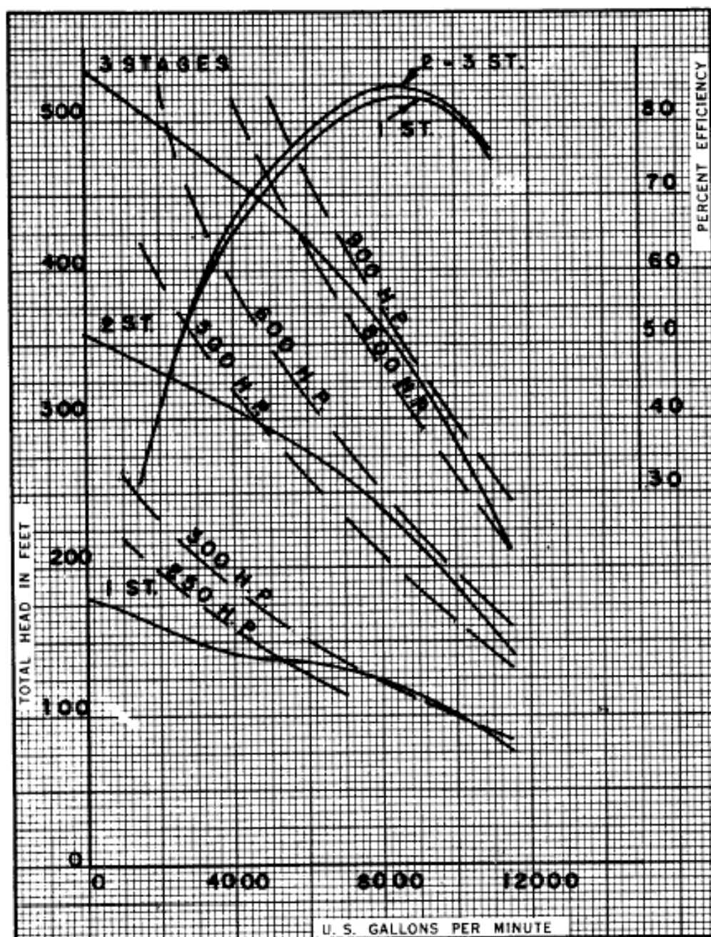
28" FIG. 6920 1170 RPM. MAXIMUM STAGES 3 IMPELLER 1213-28 BRONZE WKUXA
