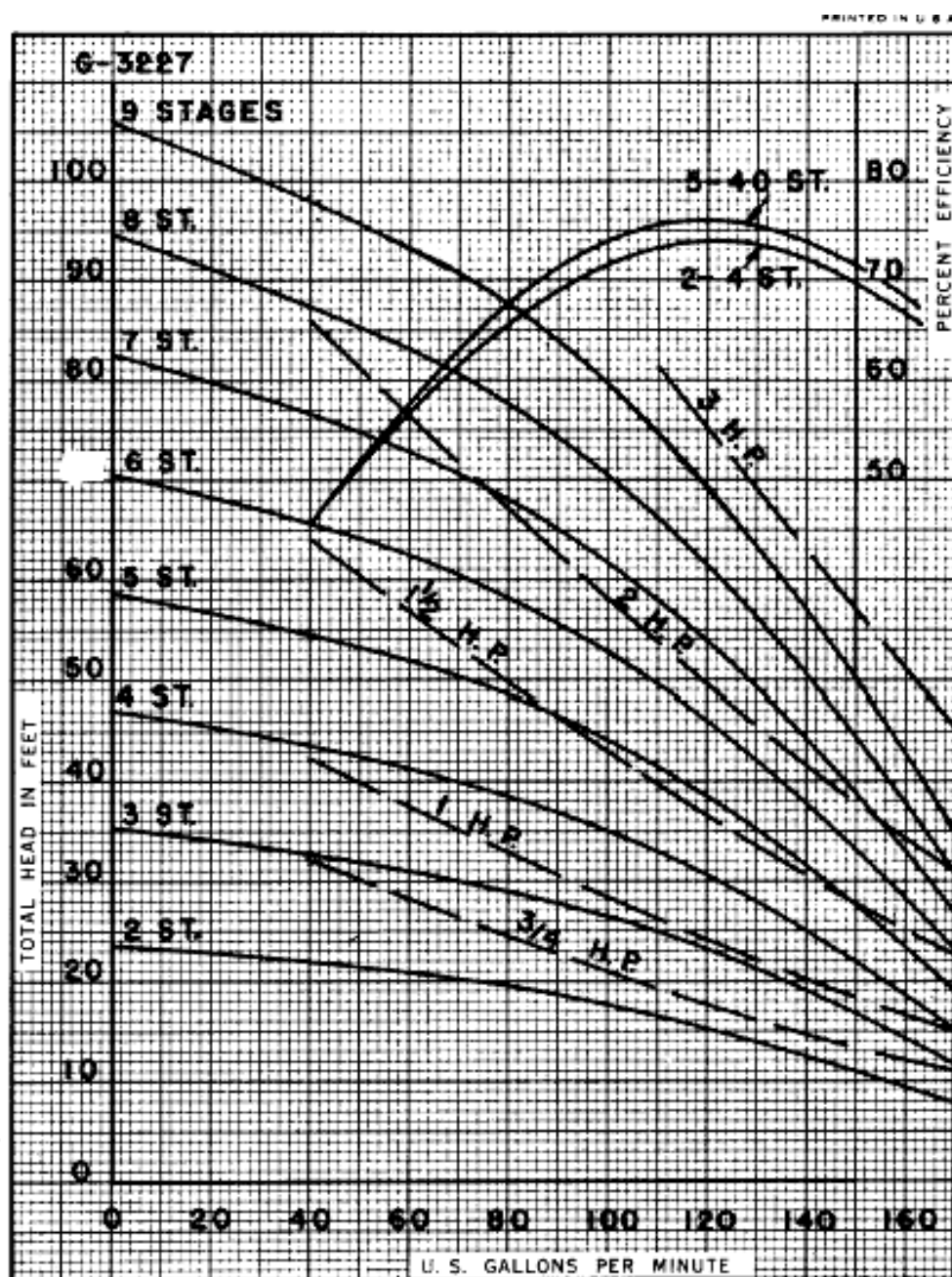
7" FIG. 6920 1160 RPM. MAXIMUM STAGES 40 IMPELLER 1072 ALL ENAMELLED WKOPZ
