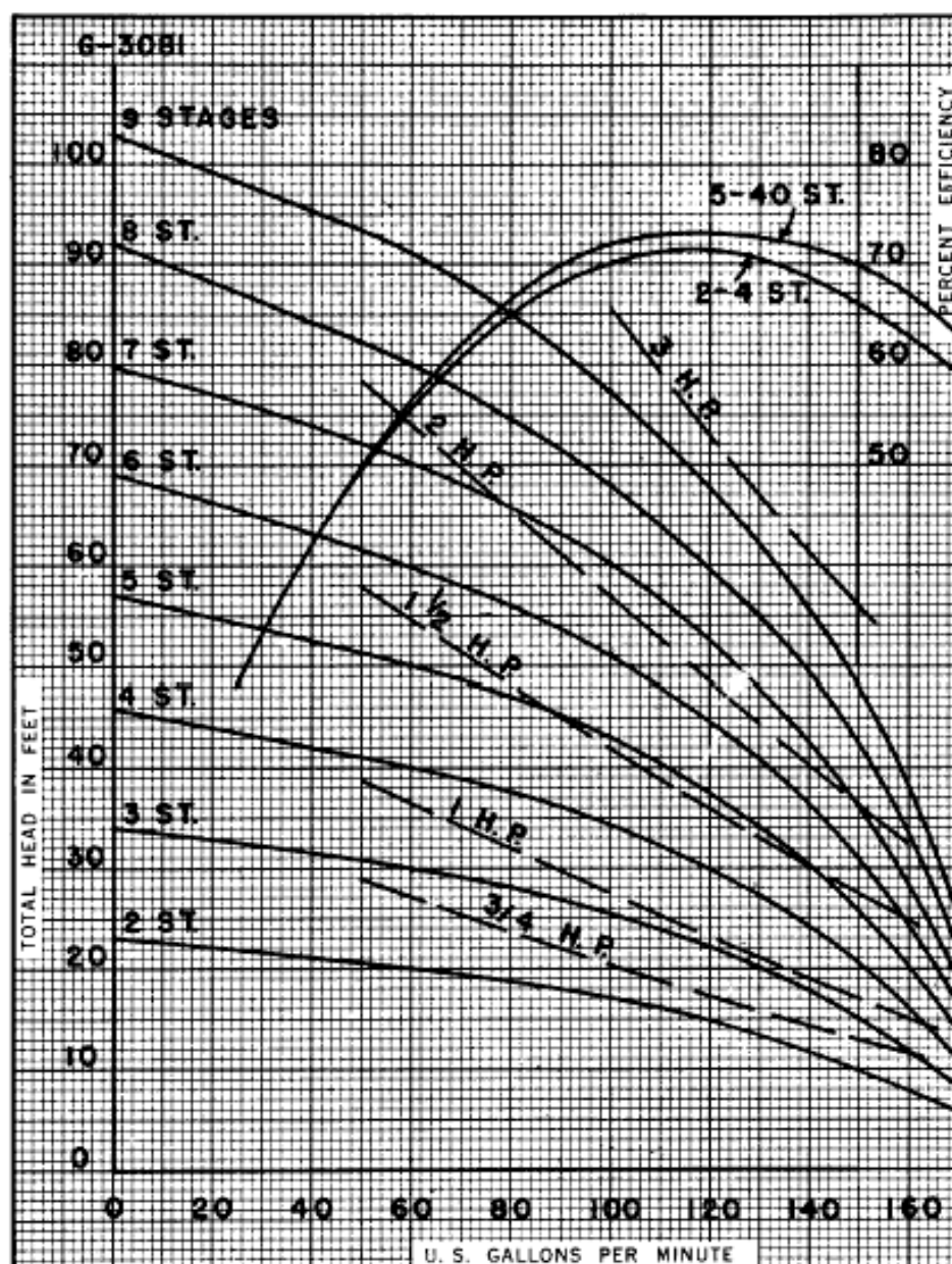
7" FIG. 6920 1160 RPM. MAXIMUM STAGES 40 IMPELLER 1072 BRONZE WKQXE
