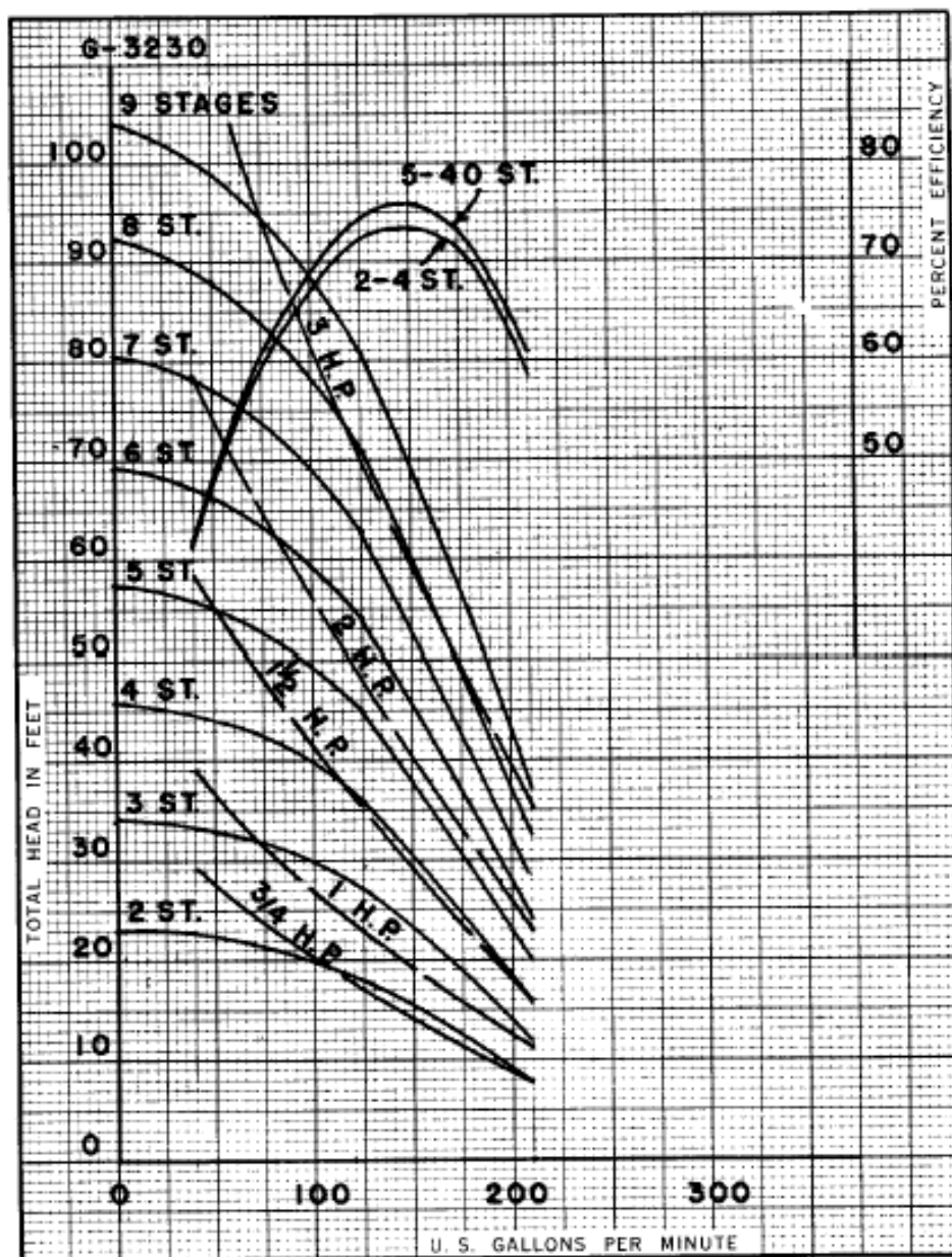
7" FIG. 6920 1160 RPM. MAXIMUM STAGES 40 IMPELLER 1073 ALL ENAMELLED WKOTC
