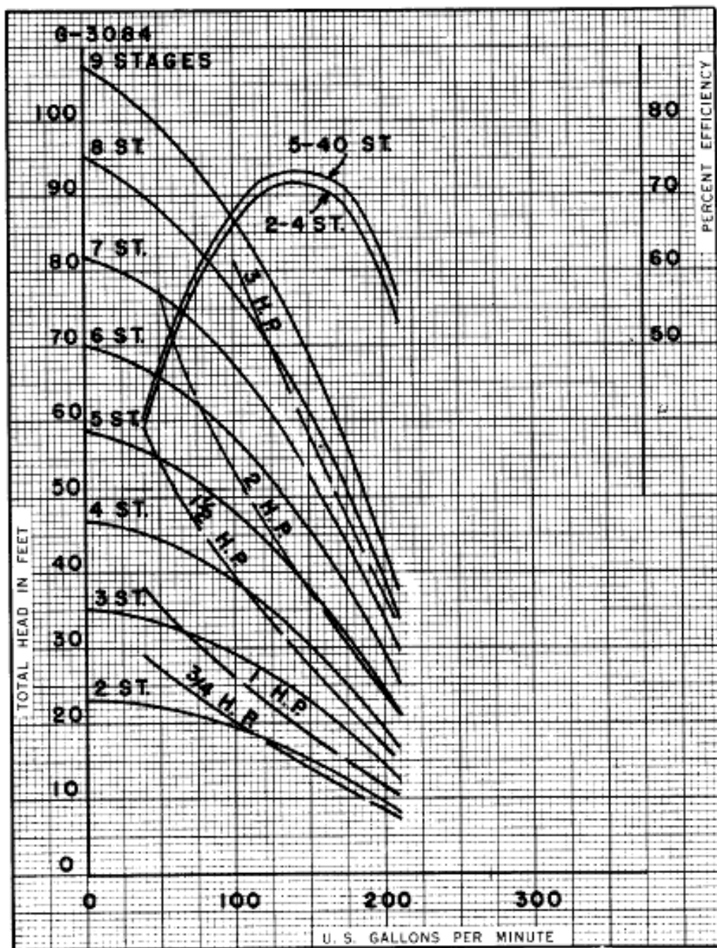
7" FIG. 6920 1160 RPM. MAXIMUM STAGES 40 IMPELLER 1073 BRONZE WKRGN
