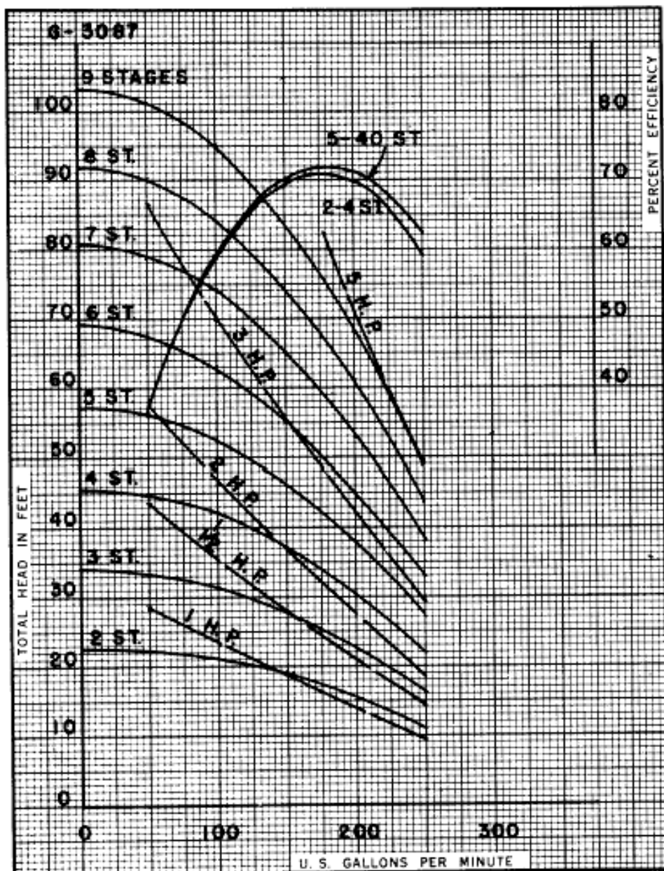
7" FIG. 6920 1160 RPM. MAXIMUM STAGES 40 IMPELLER 1074 BRONZE WKRJQ
