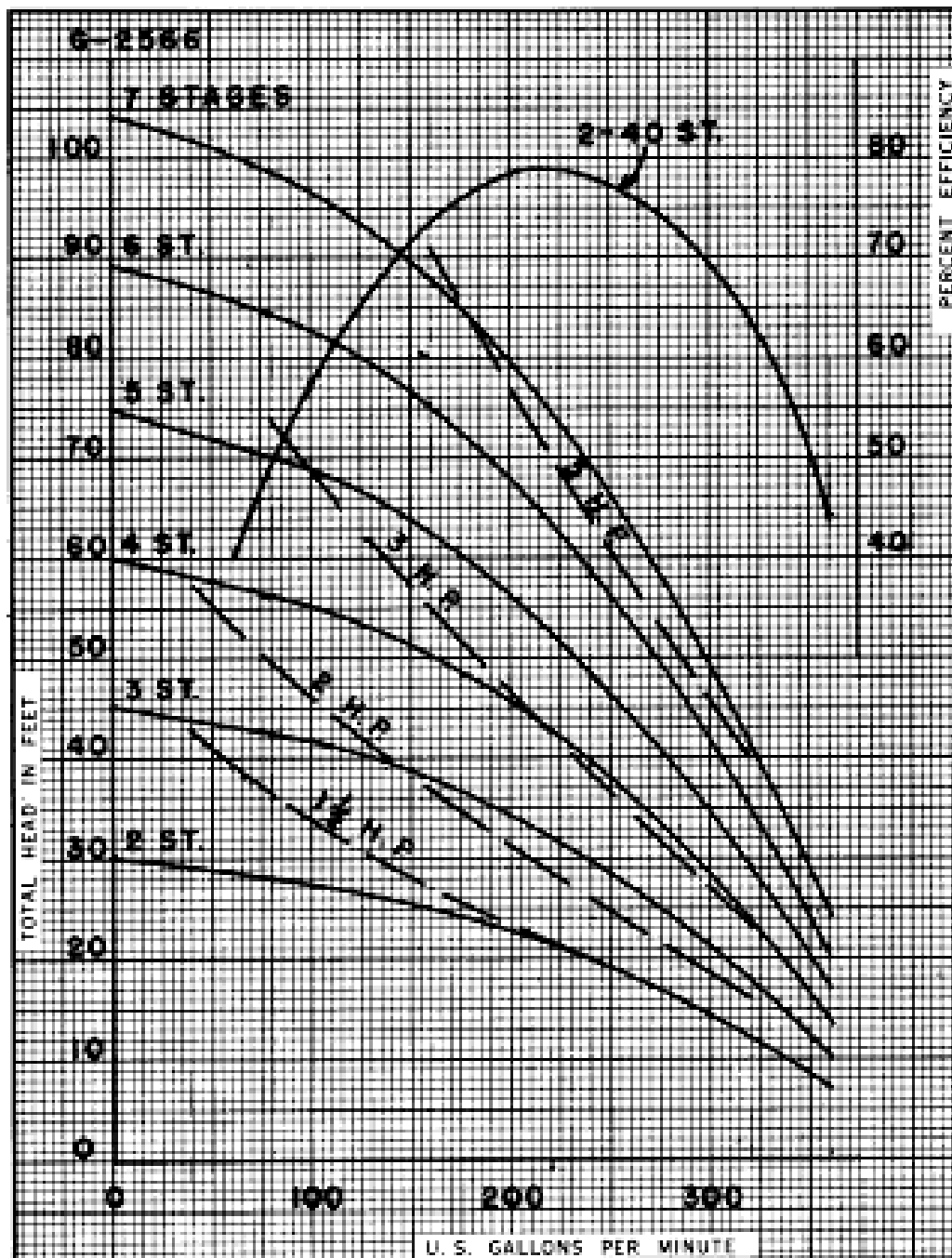
8" FIG. 6920 1160 RPM MAXIMUM STAGES 40 IMPELLER 1113 ALL ENAMELLED WKWPR
