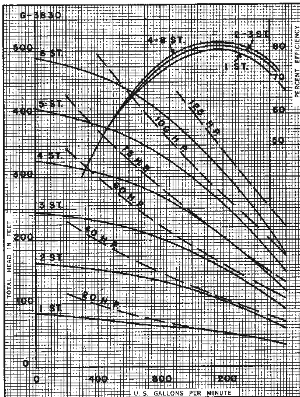
12" FIG. 6920 1750 RPM. MAXIMUM STAGES 8 IMPELLER 1133 ALL ENAMELLED WPJKD
