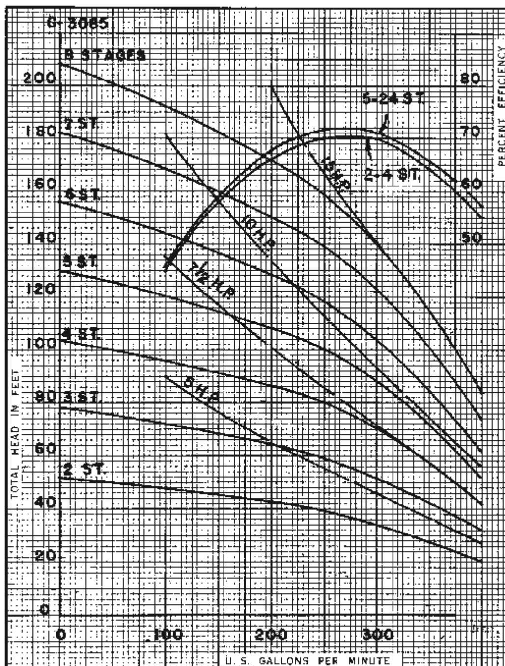
7" FIG. 6920 1750 RPM. MAXIMUM STAGES 24 IMPELLER 1074 BRONZE WKRHO
