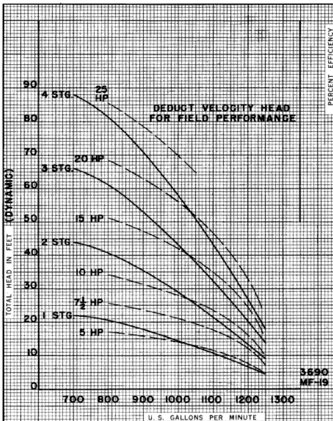
Figure 6340 Performance 6 Inch Niagara Junior Propeller Pumps
