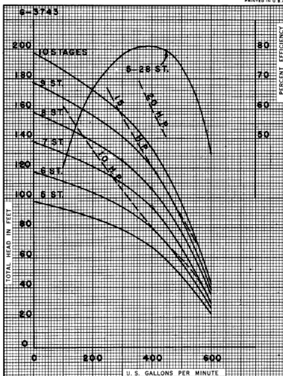
12" FIG. 6920 870 RPM. MAXIMUM STAGES 28 IMPELLER 745 ALL ENAMELLED WKNZJ
