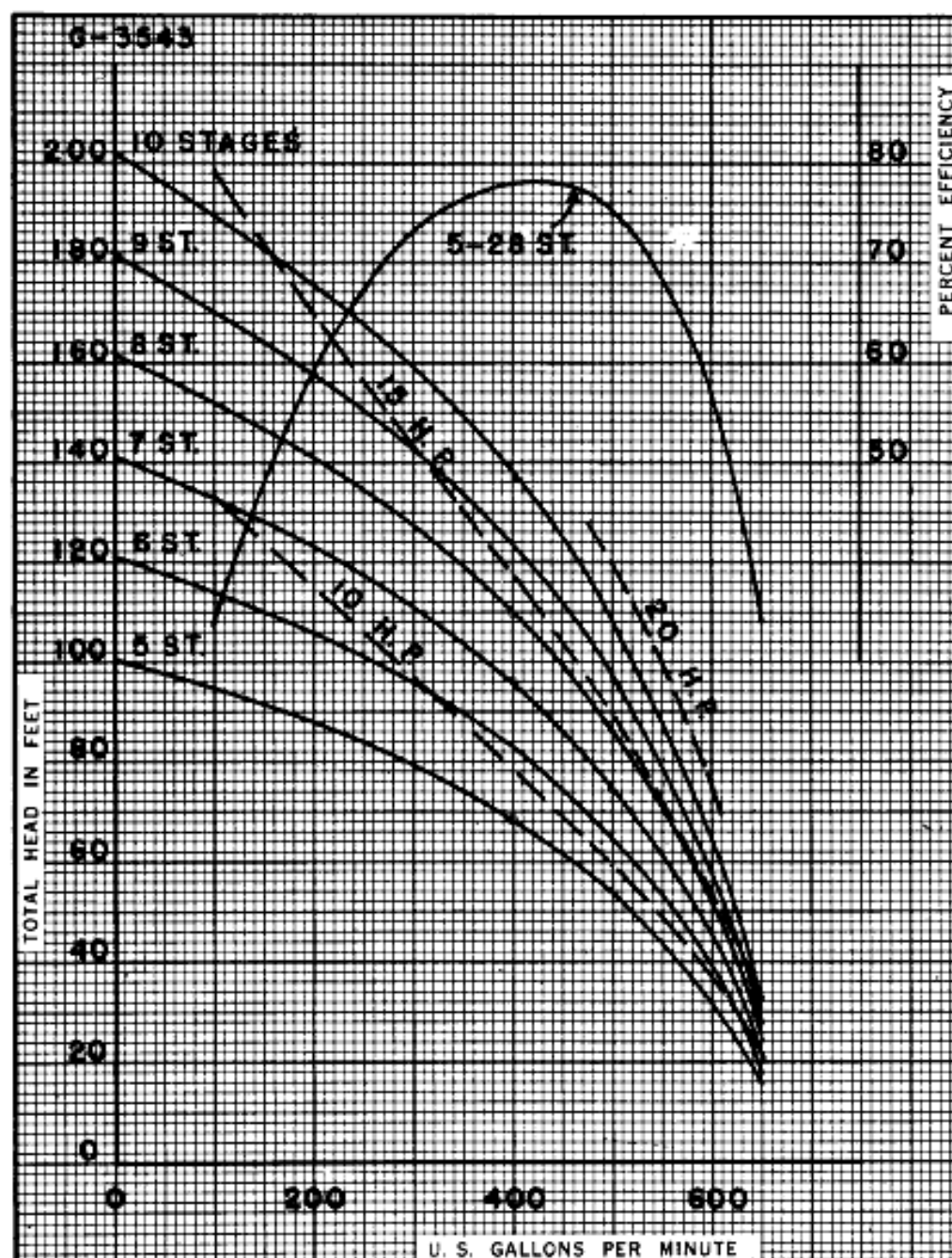
12" FIG. 6920 870 RPM. MAXIMUM STAGES 28 IMPELLER 745 BRONZE WKWXZ
