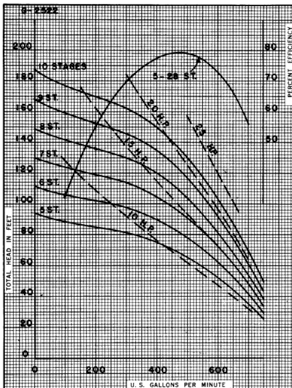
12" FIG. 6920 870 RPM. MAXIMUM STAGES 28 IMPELLER 747 BRONZE WKUJN
