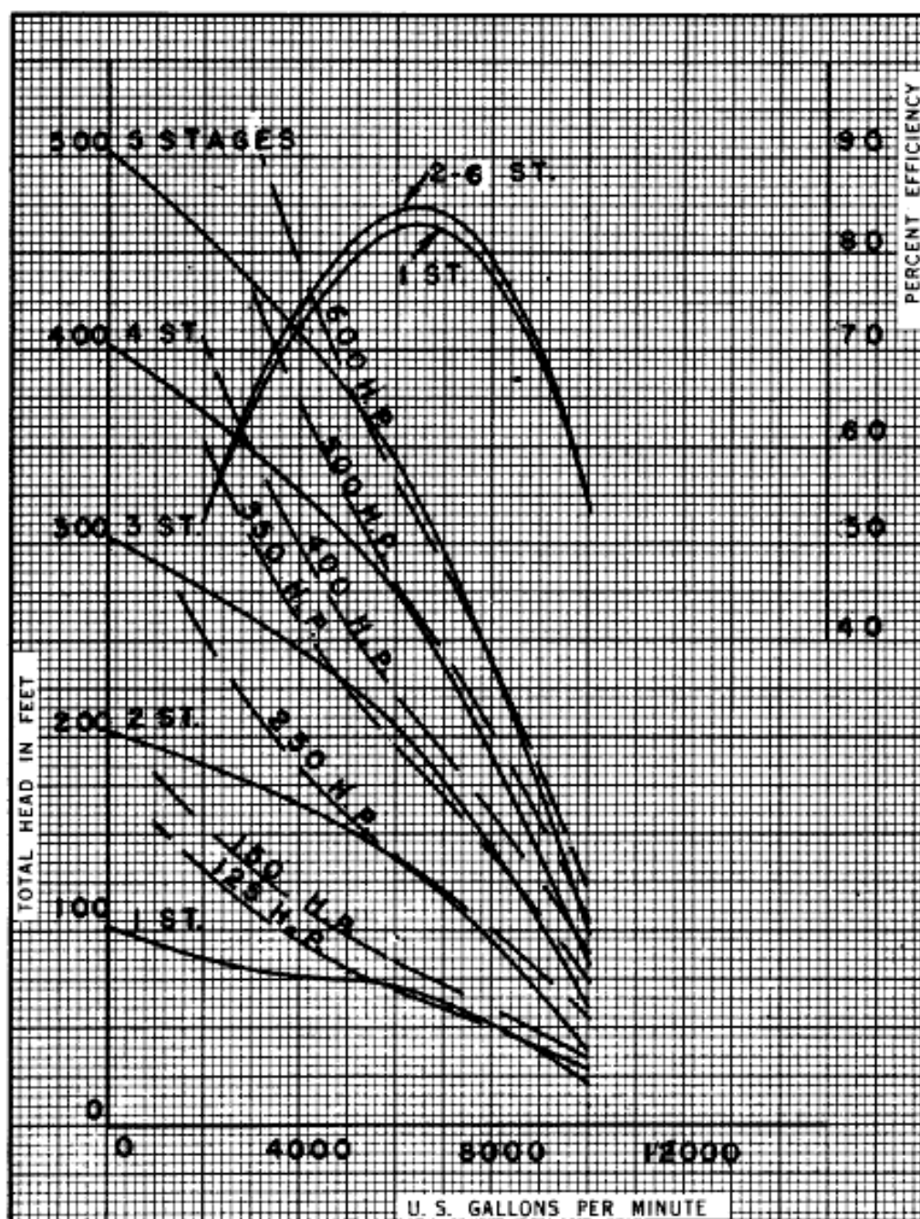
28" FIG. 6920 880 RPM. MAXIMUM STAGES 6 IMPELLER 1213-28 BRONZE W KUYB
