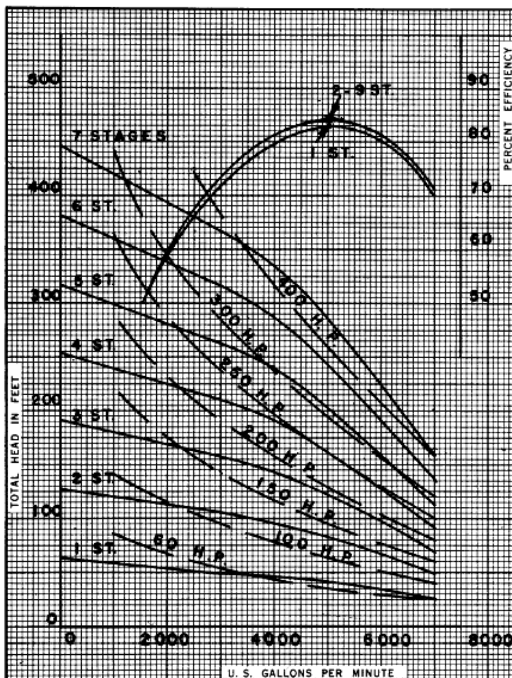
28" FIG. 6920 700 RPM. MAXIMUM STAGES 9 IMPELLER 1213-28 BRONZE WKU2C
