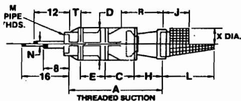
STANDARD DIMENSIONS
