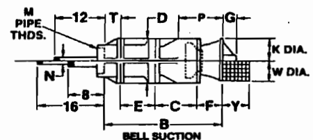
STANDARD DIMENSIONS
