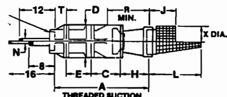
STANDARD DIMENSIONS
