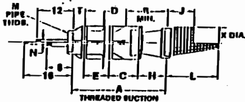
STANDARD DIMENSIONS
