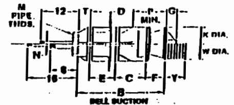
STANDARD DIMENSIONS
