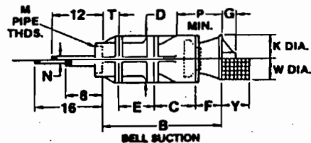
STANDARD DIMENSIONS
