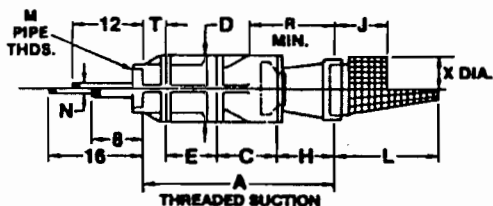
STANDARD DIMENSIONS
