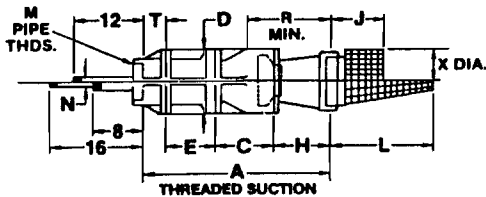
STANDARD DIMENSIONS
