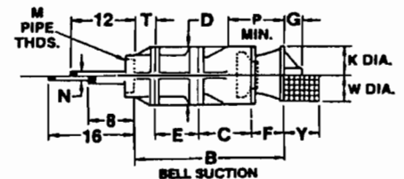
STANDARD DIMENSIONS
