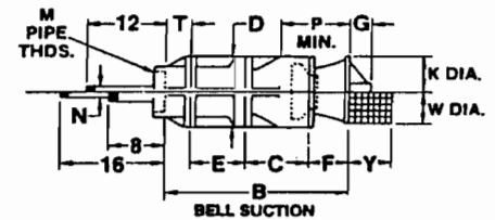
STANDARD DIMENSIONS
