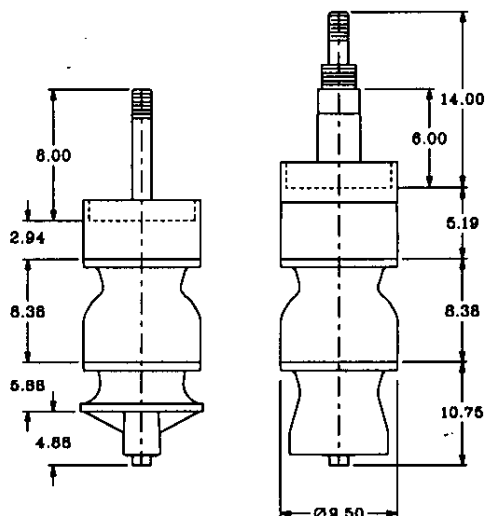
OPEN LINESHAFT
