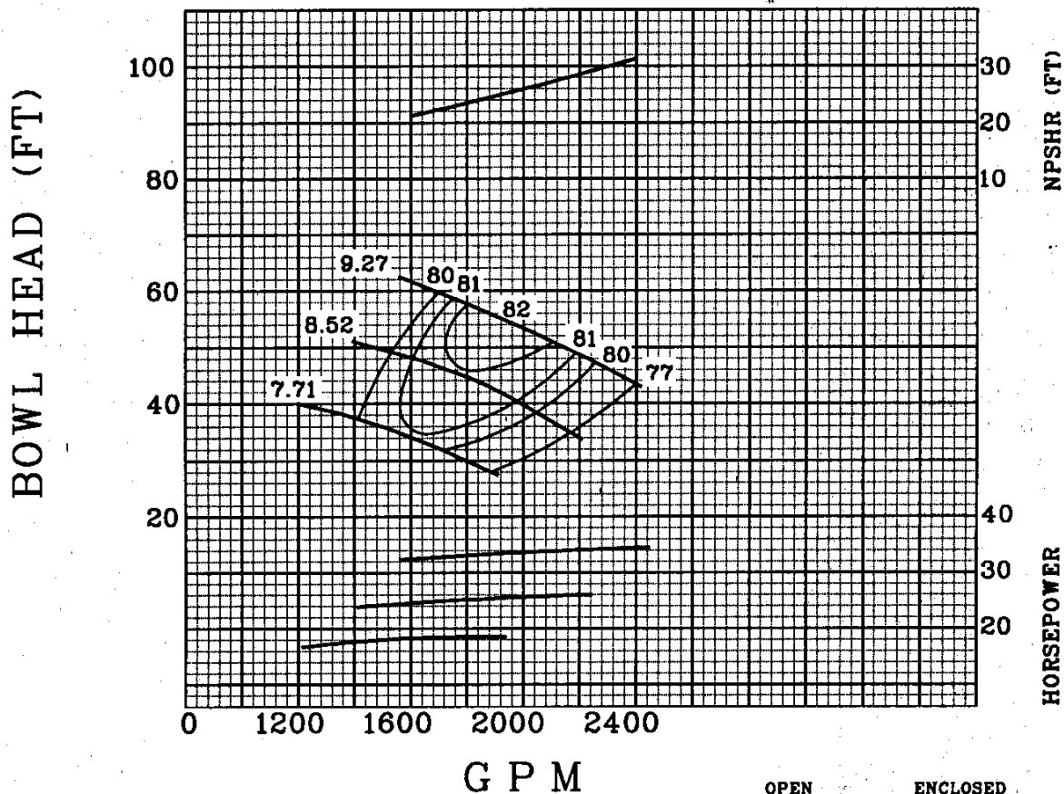
OPEN LINESHAFT
