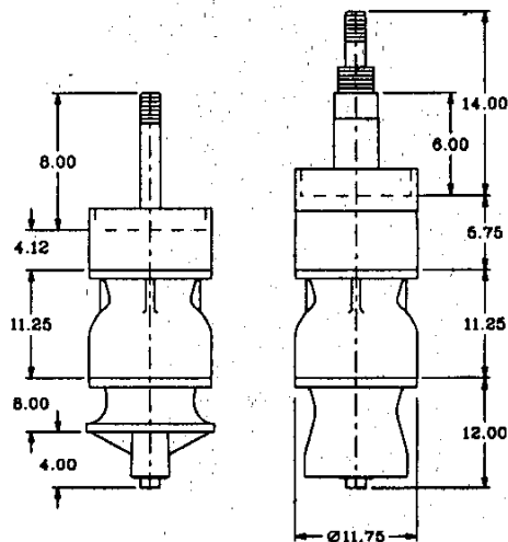
OPEN LINESHAFT
