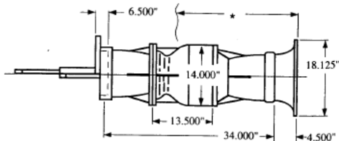
LINESHAFT TURBINE
