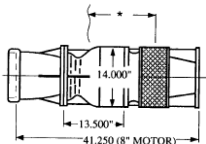
SUBMERSIBLE TURBINE
