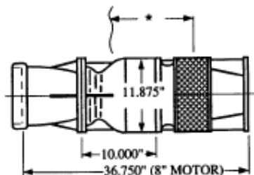
SIMFLO TURBINE
