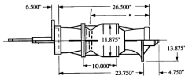
LINESHAFT TURBINE
