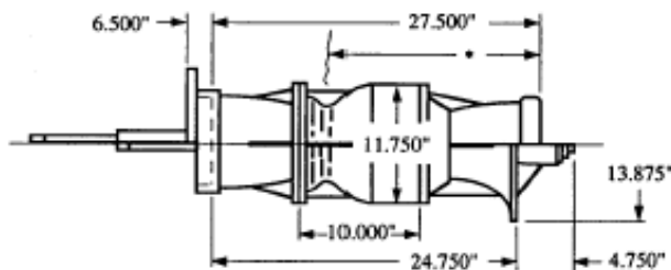
LINESHAFT TURBINE
