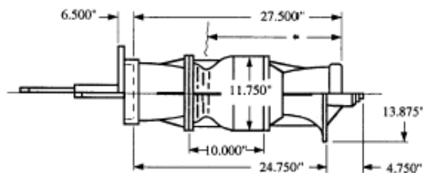
IN-SHAFT TURBINE
