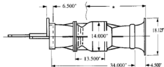
LINESHAFT TURBINE
