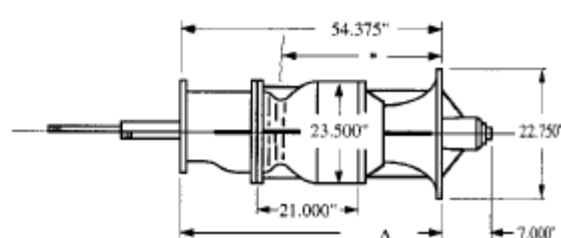
LINESHAFT TURBINE
