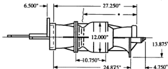
IN-SHAFT TURBINE
