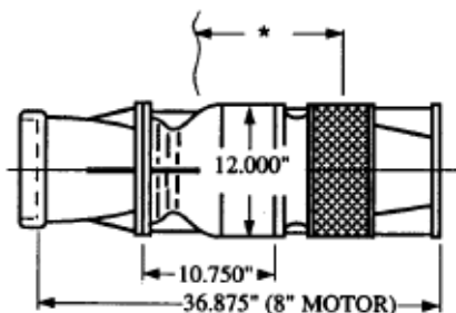
SUBMERSIBLE TURBINE
