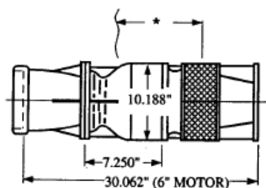
SUBMERSIBLE TURBINE
