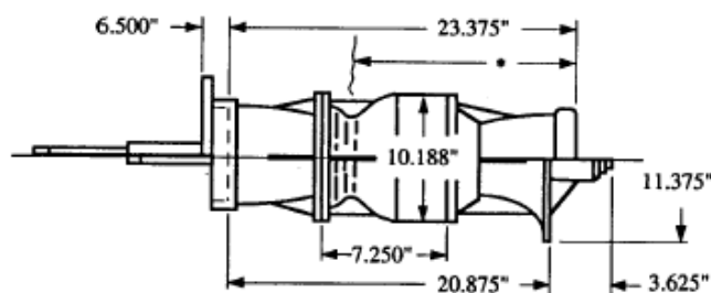
LINESHAFT TURBINE
