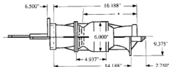
LINESHAFT TURBINE
