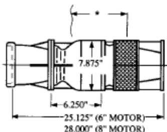
SUBMERSIBLE TURBINE
