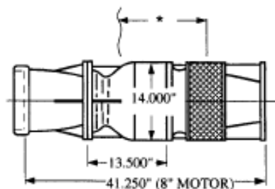
SUBMERSIBLE TURBINE
