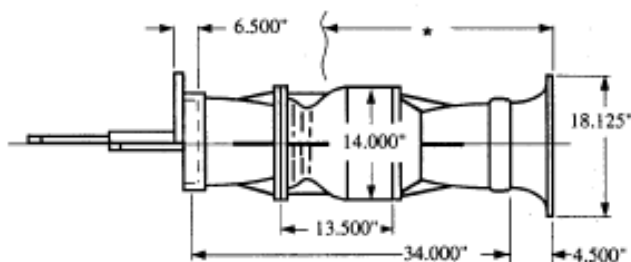
LINESHAFT TURBINE
