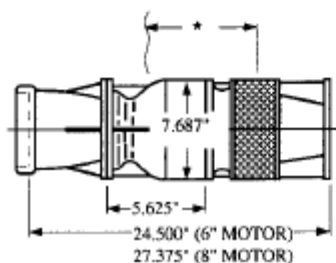
SUBMERSIBLE TURBINE
