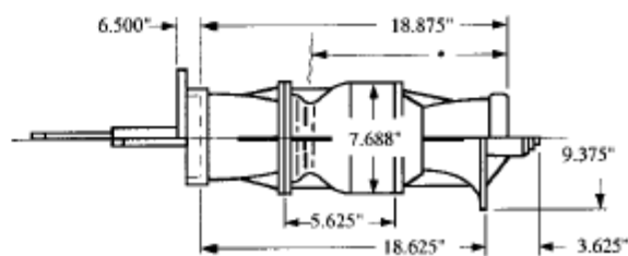
LINESHAFT TURBINE
