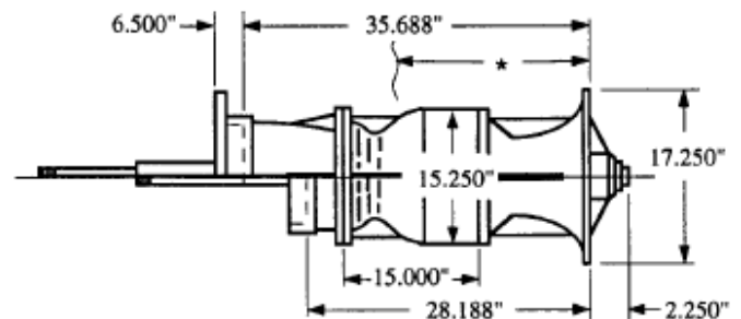
LINESHAFT TURBINE
